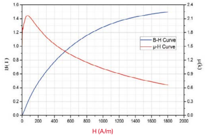
The B-H Curve and \mu -H Curve of Amorphous CACC Cores
