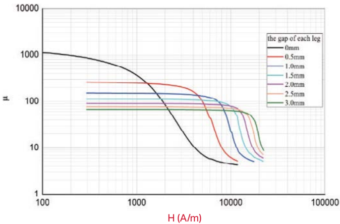
The DC-Bias Curve of Amorphous CACC Cores
