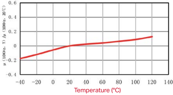
Relative change of \mu vs temperature
