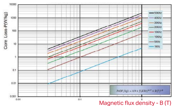
Iron-based Amorphous CACC Series Core Loss Curve
