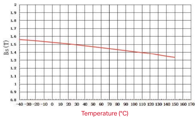
Amorphous relative change of B_s VS Temperature
